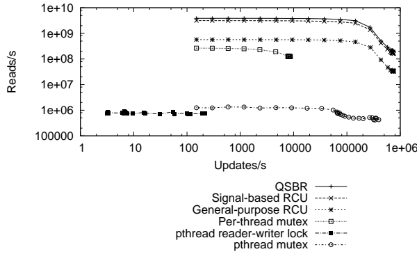
Fig. 10. Update Overhead, 64-core POWER5+, Logarithmic Scale
