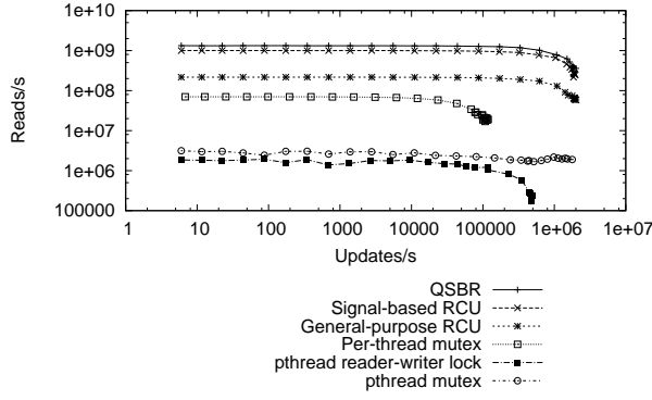
Fig. 9. Update Overhead, 8-core Intel Xeon, Logarithmic Scale
